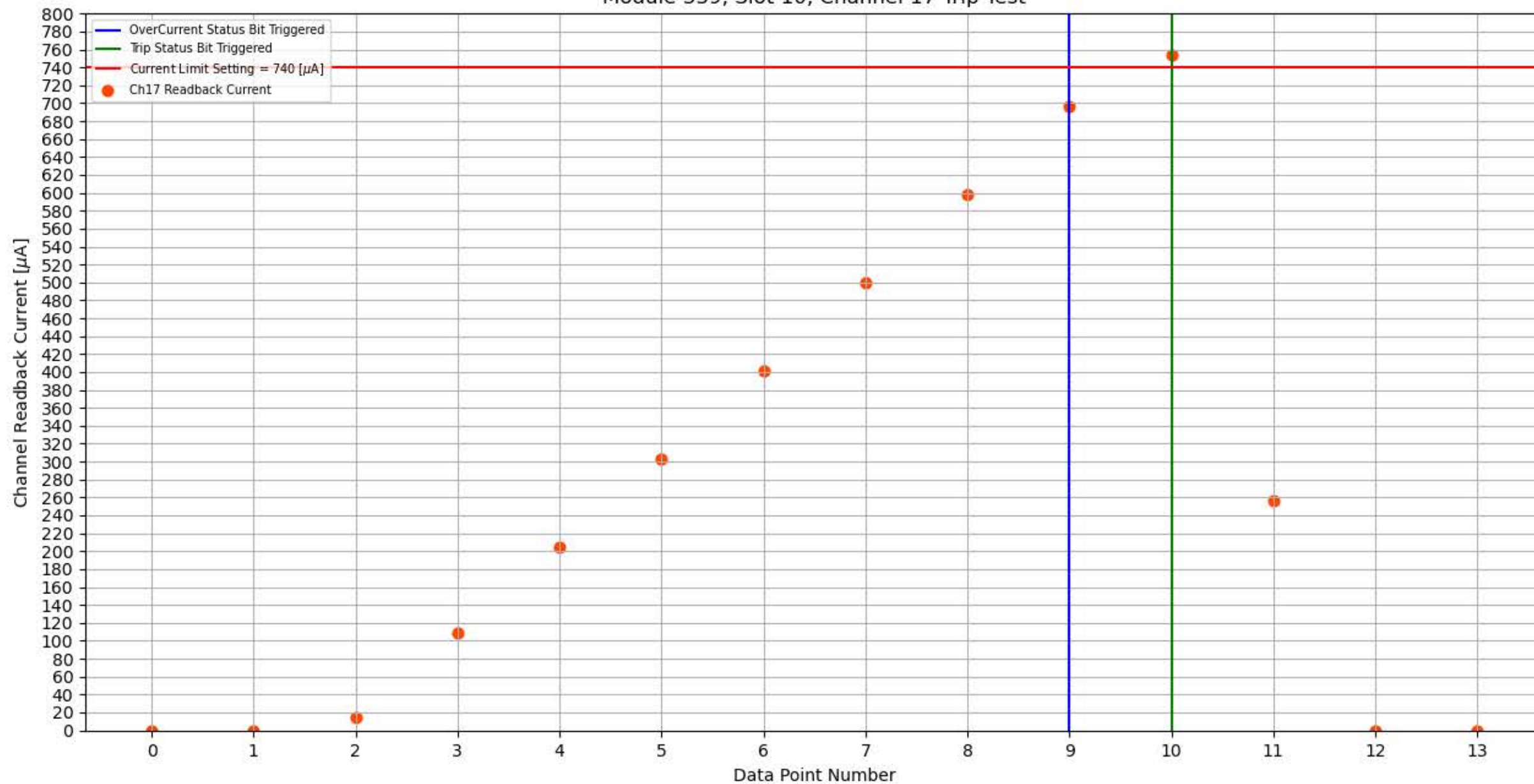
Module 339, Slot 10, Channel 17 Trip Test
