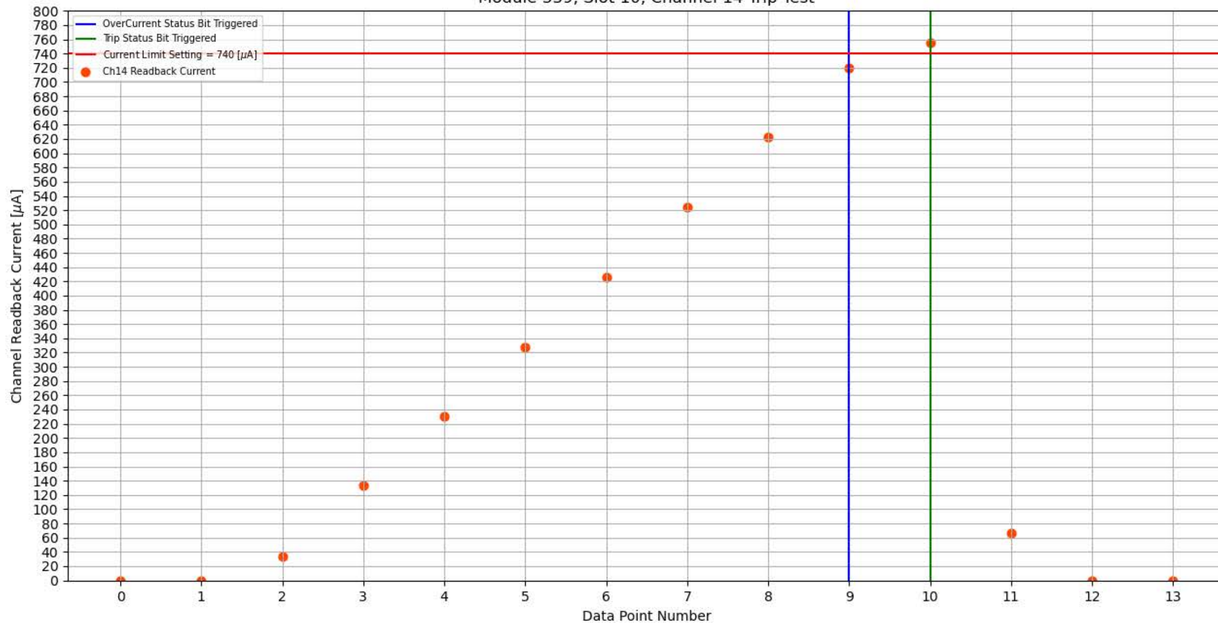
Module 339, Slot 10, Channel 14 Trip Test
