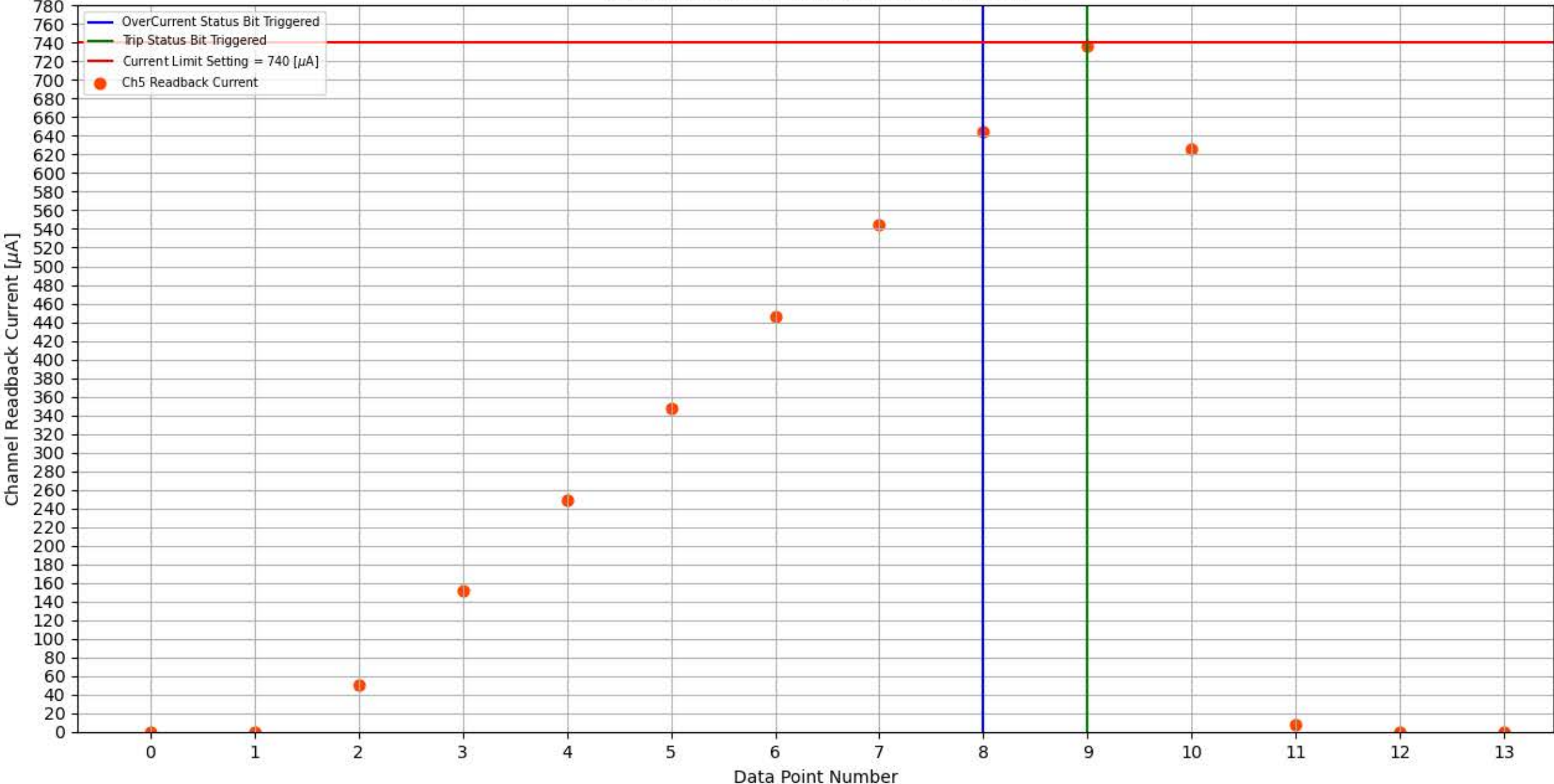
Module 339, Slot 10, Channel 5 Trip Test
