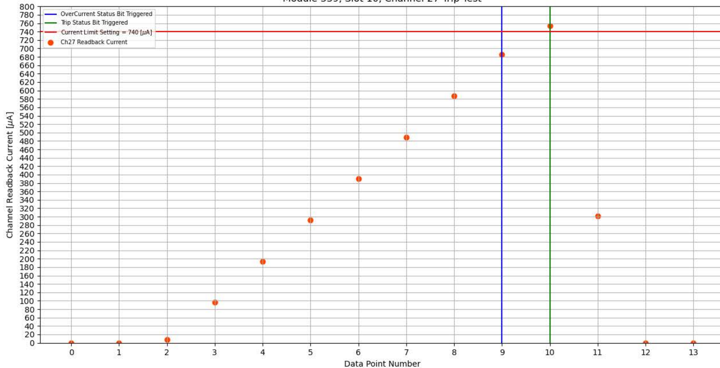
Module 339, Slot 10, Channel 27 Trip Test
