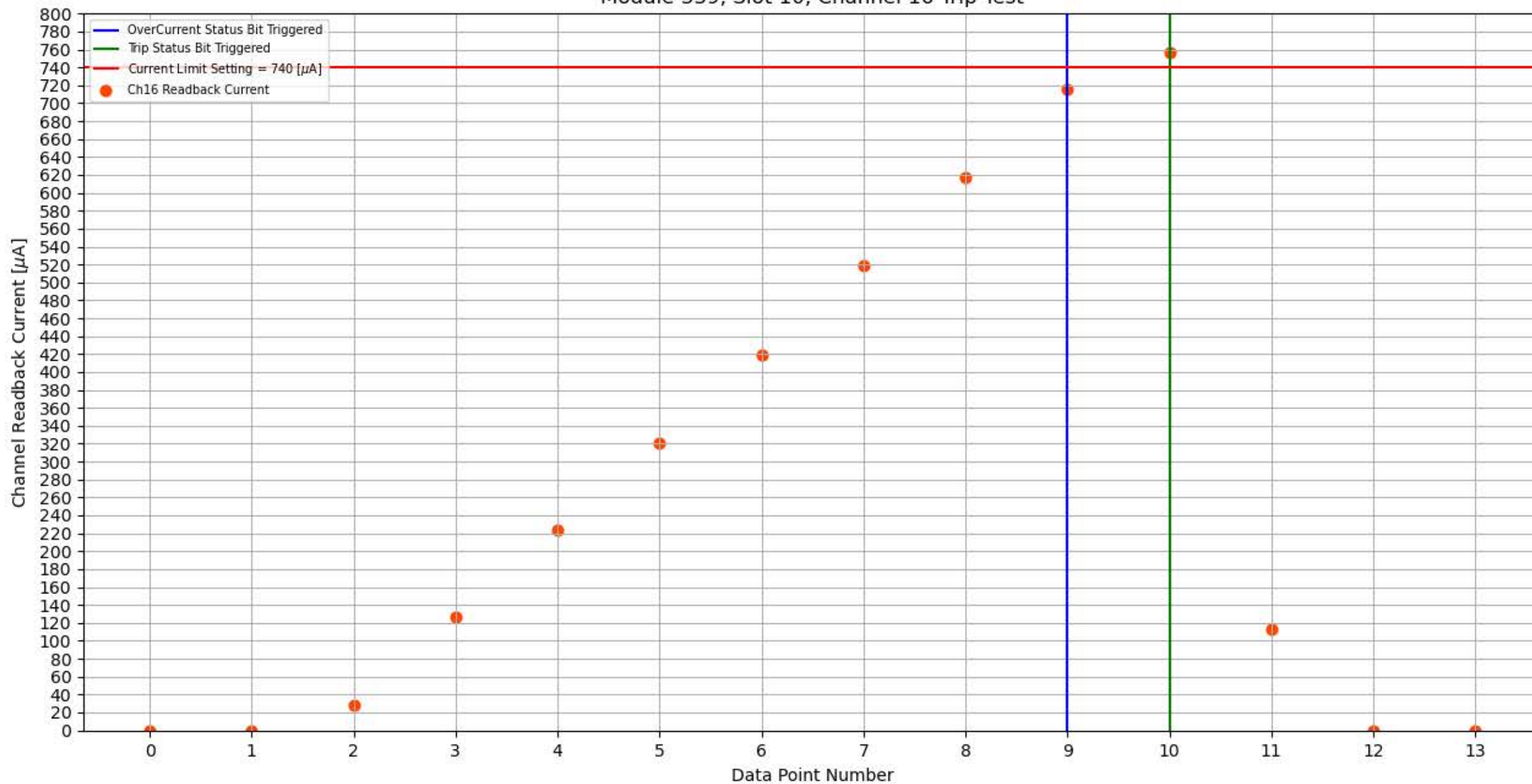
Module 339, Slot 10, Channel 16 Trip Test
