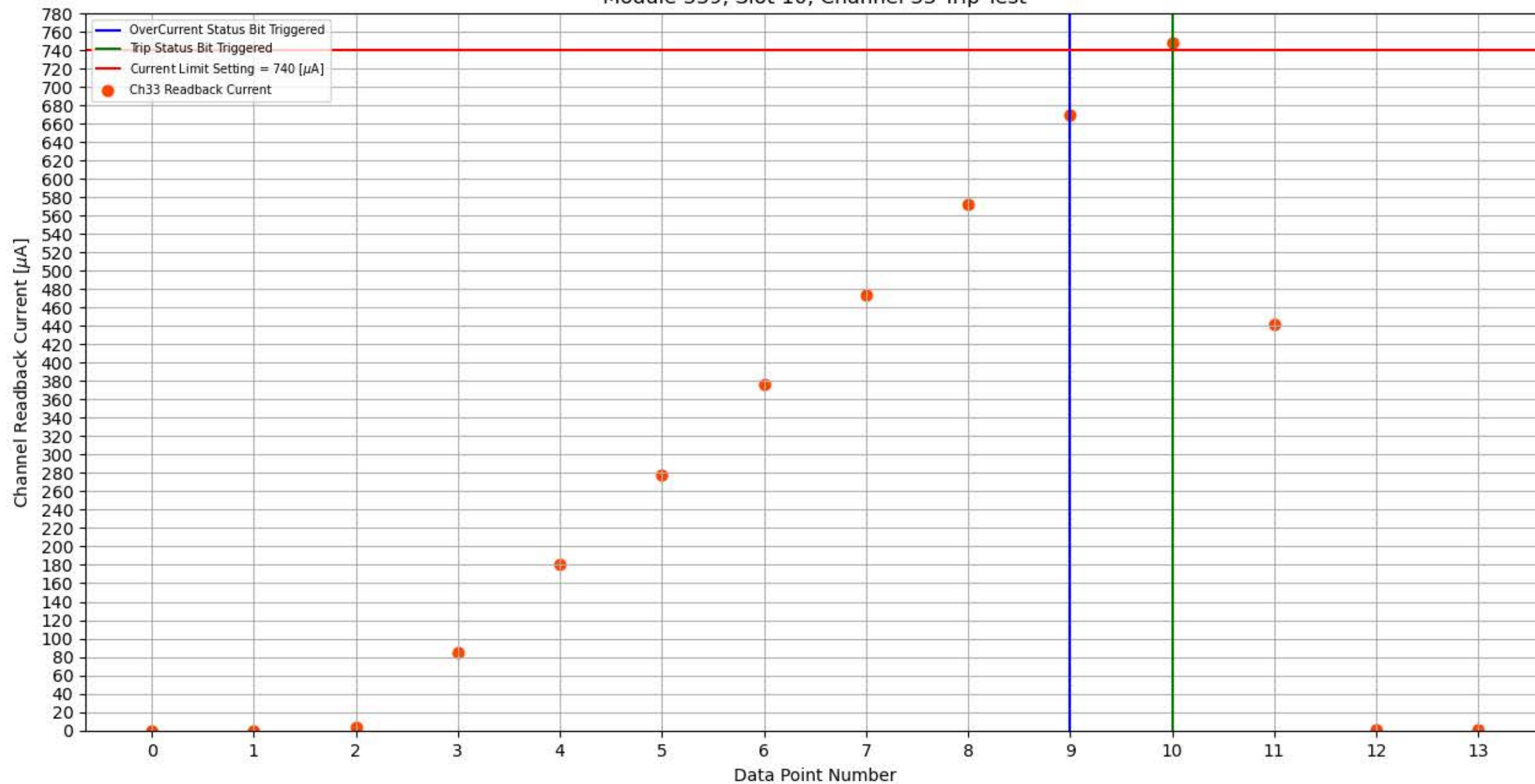
Module 339, Slot 10, Channel 33 Trip Test
