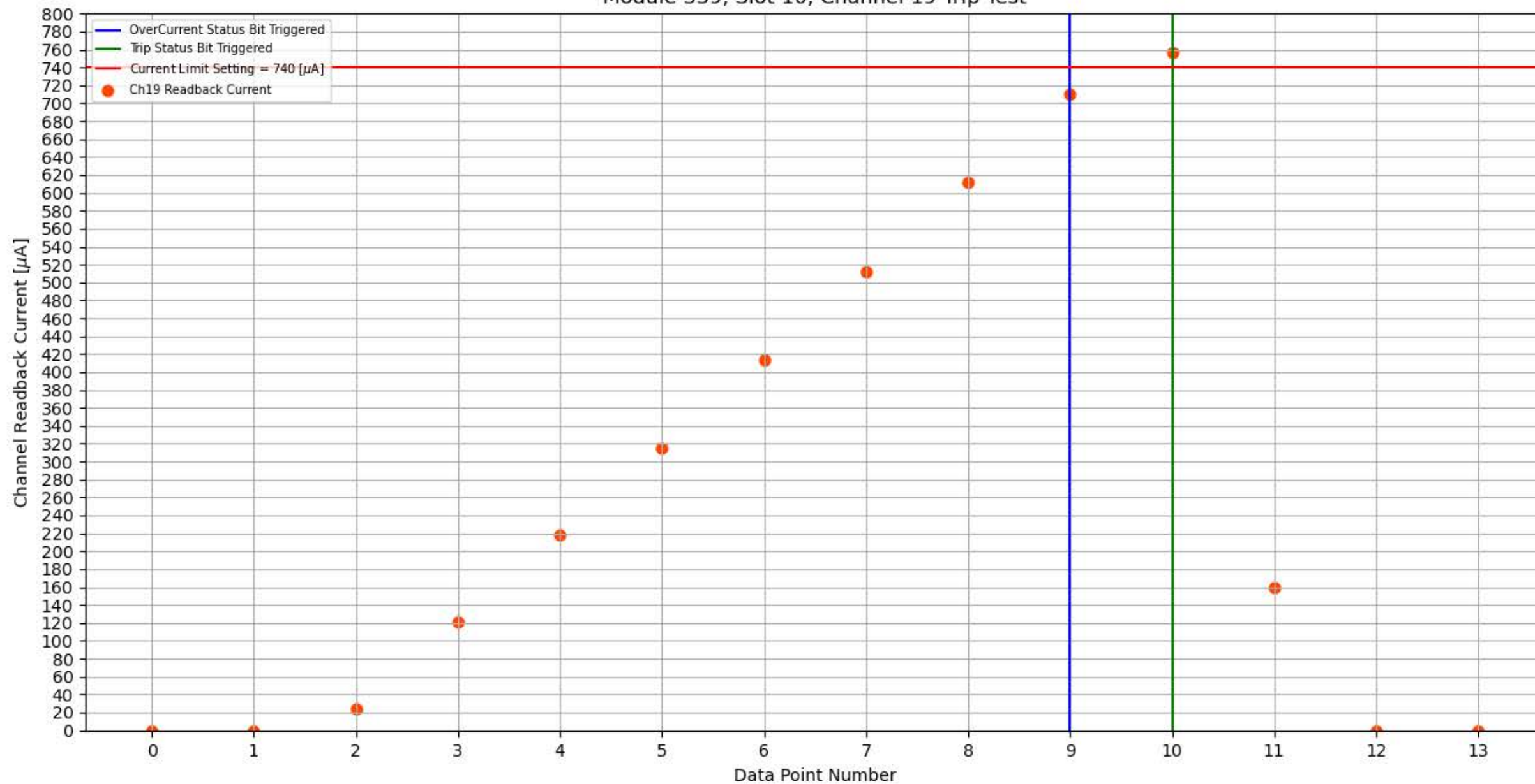
Module 339, Slot 10, Channel 19 Trip Test
