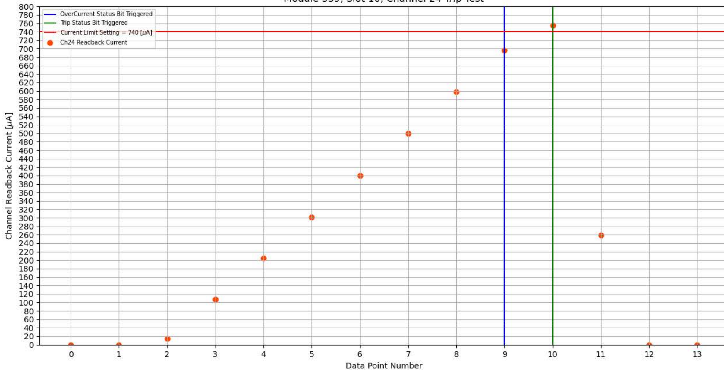
Module 339, Slot 10, Channel 24 Trip Test
