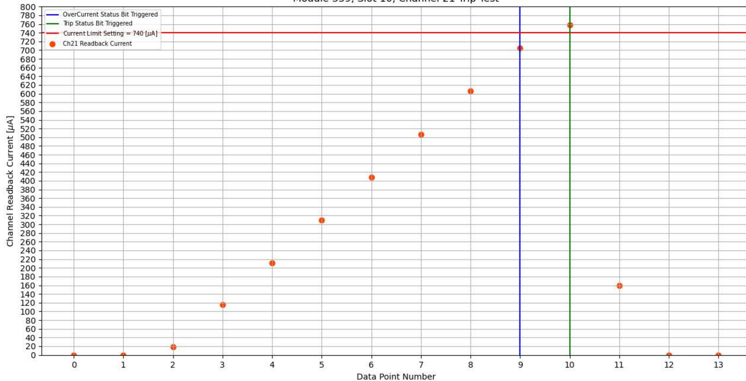
Module 339, Slot 10, Channel 21 Trip Test
