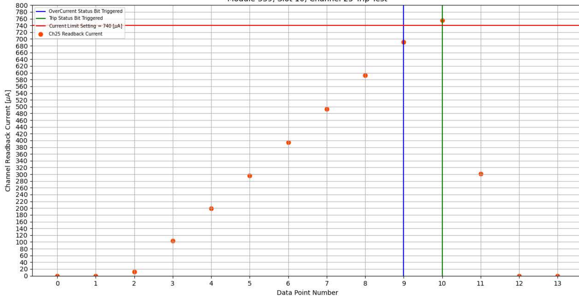
Module 339, Slot 10, Channel 25 Trip Test
