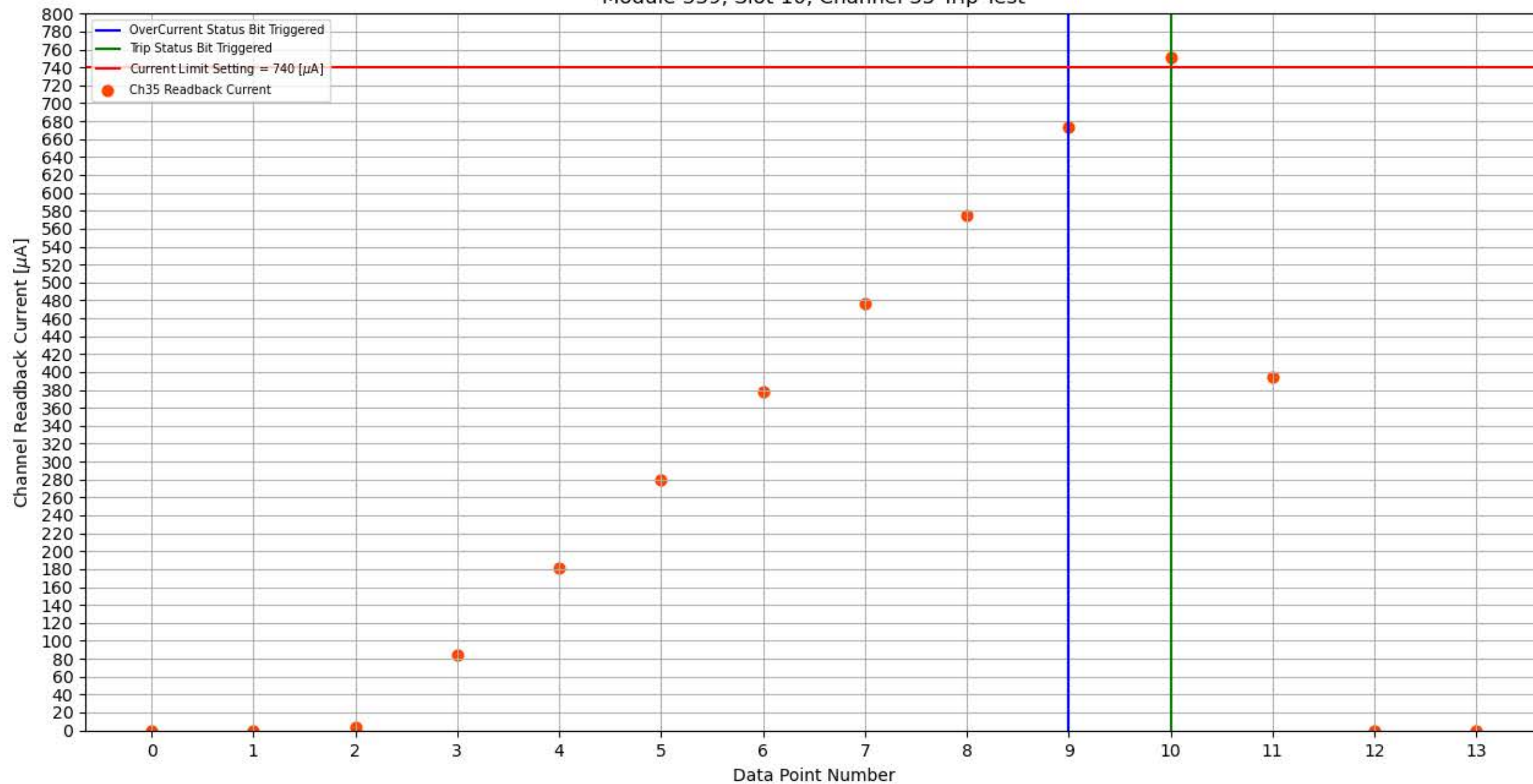
Module 339, Slot 10, Channel 35 Trip Test
