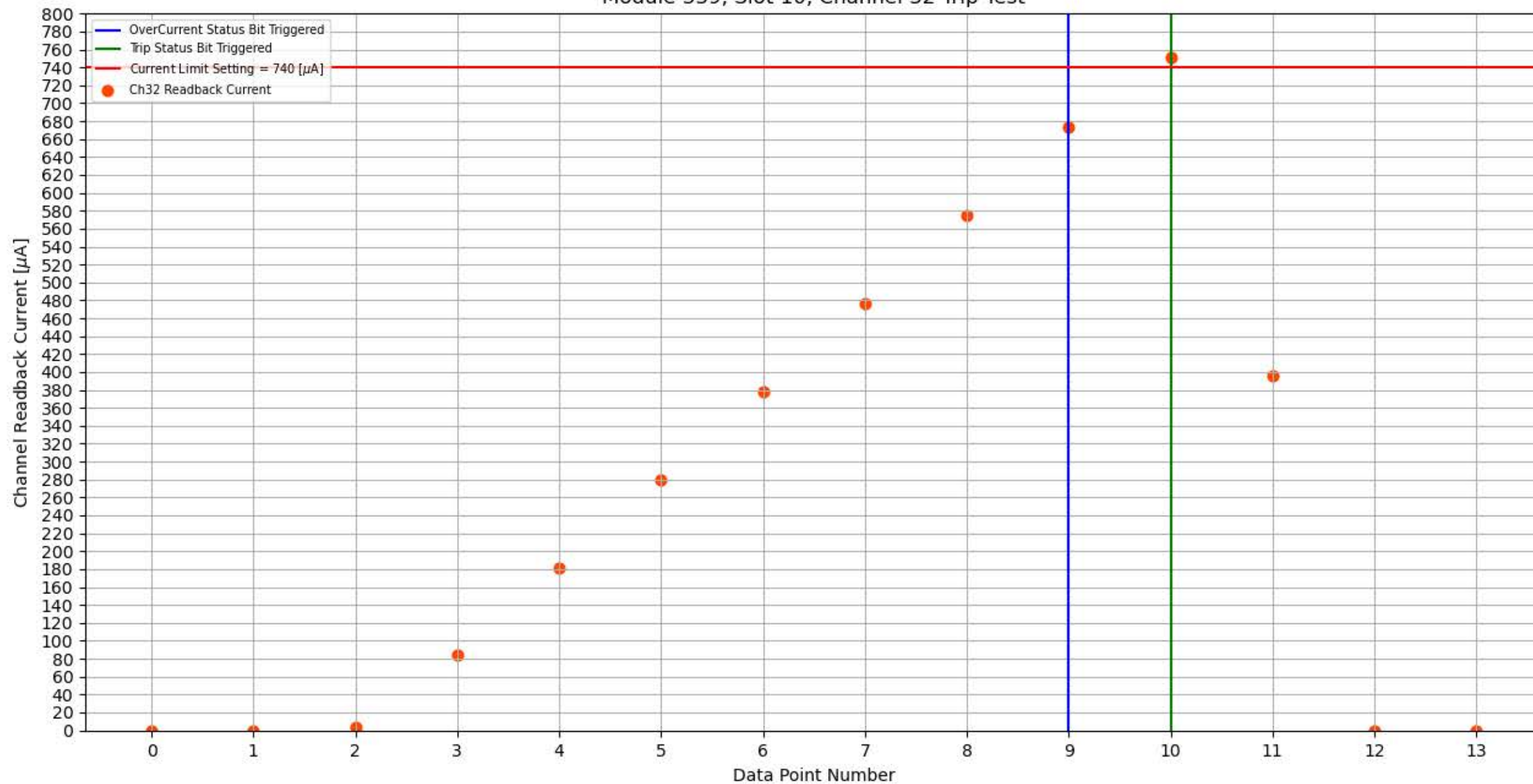
Module 339, Slot 10, Channel 32 Trip Test
