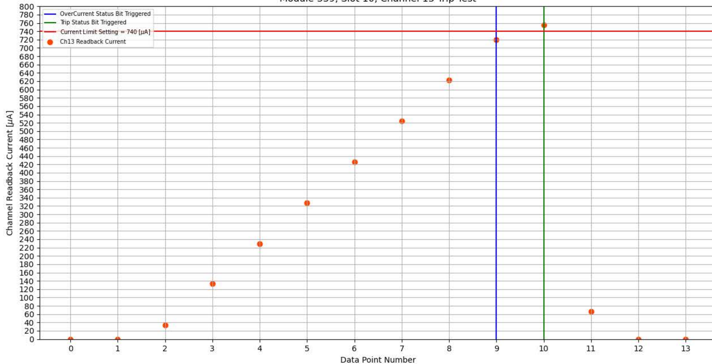
Module 339, Slot 10, Channel 13 Trip Test
