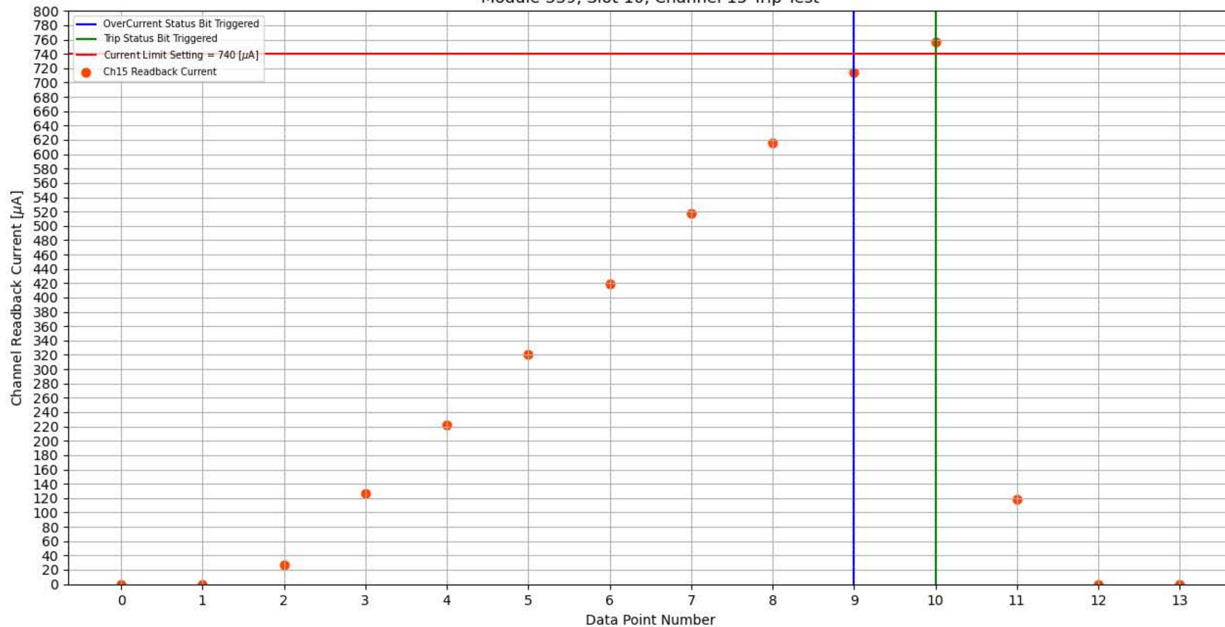
Module 339, Slot 10, Channel 15 Trip Test
