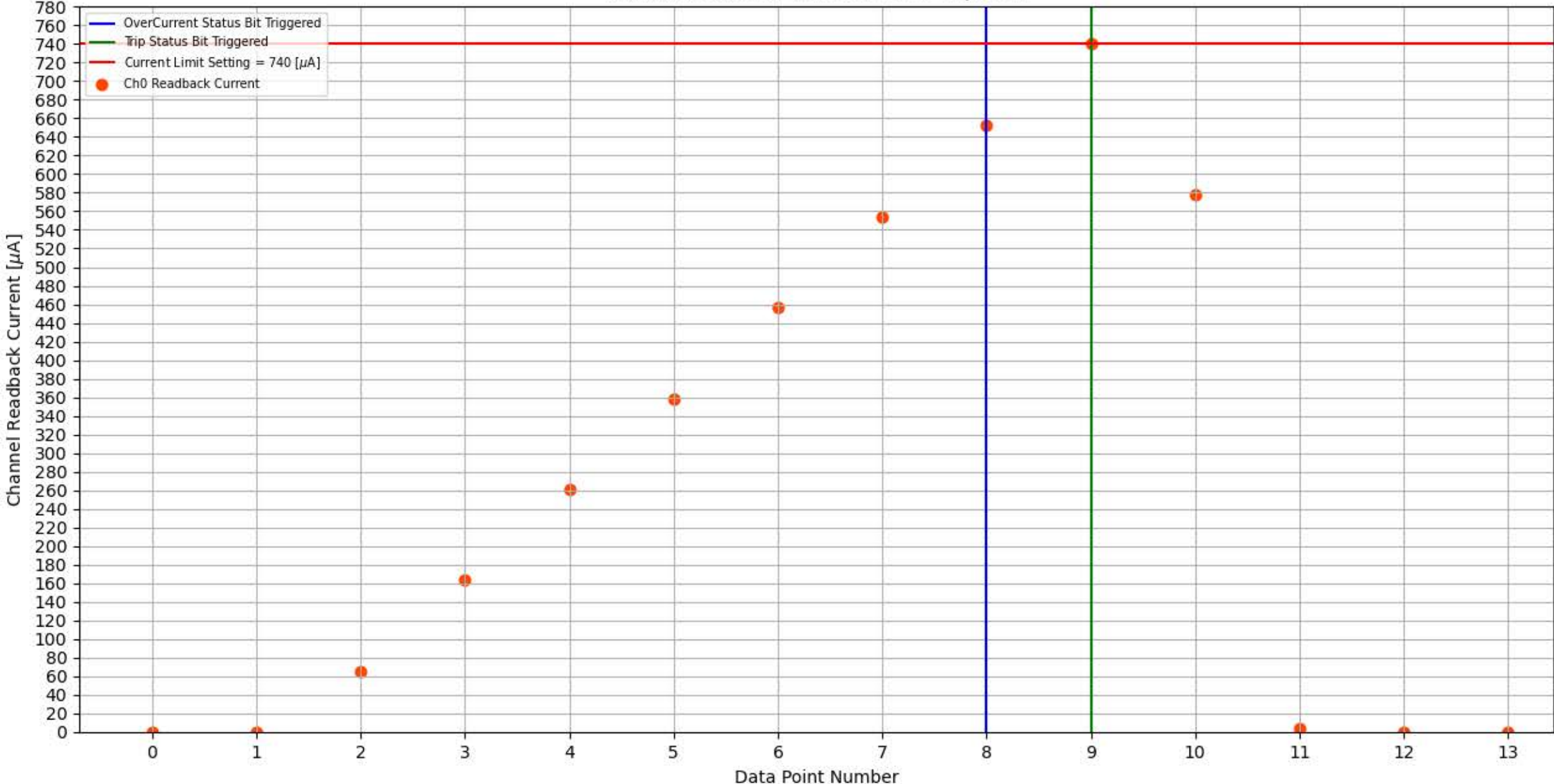
Module 339, Slot 10, Channel 0 Trip Test
