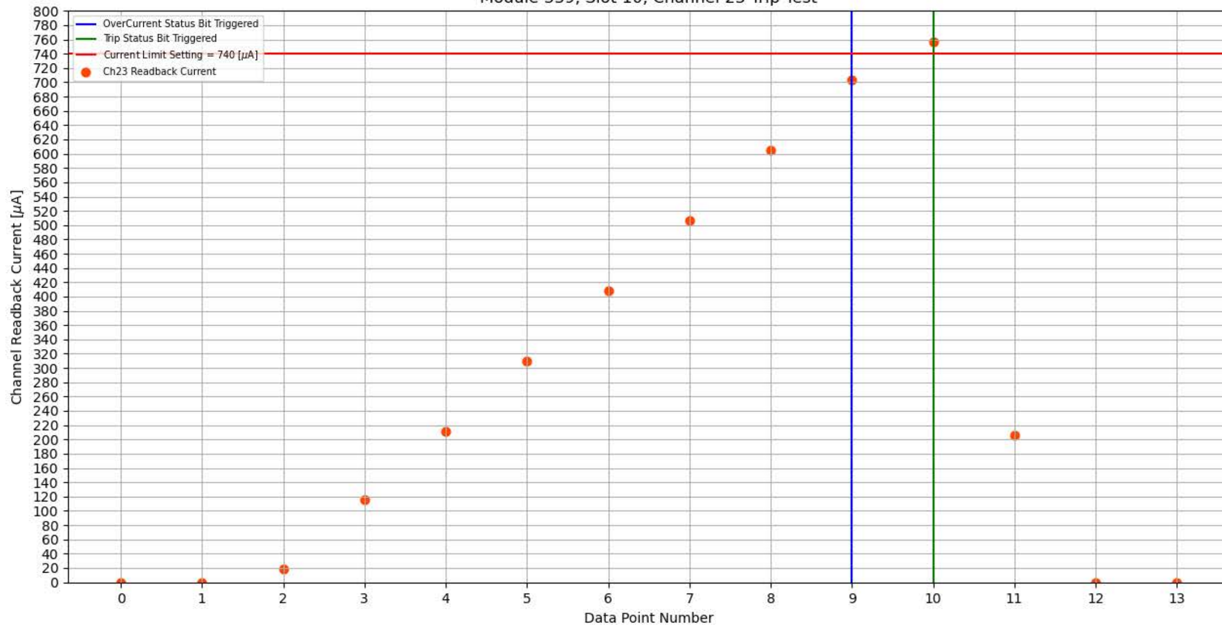
Module 339, Slot 10, Channel 23 Trip Test
