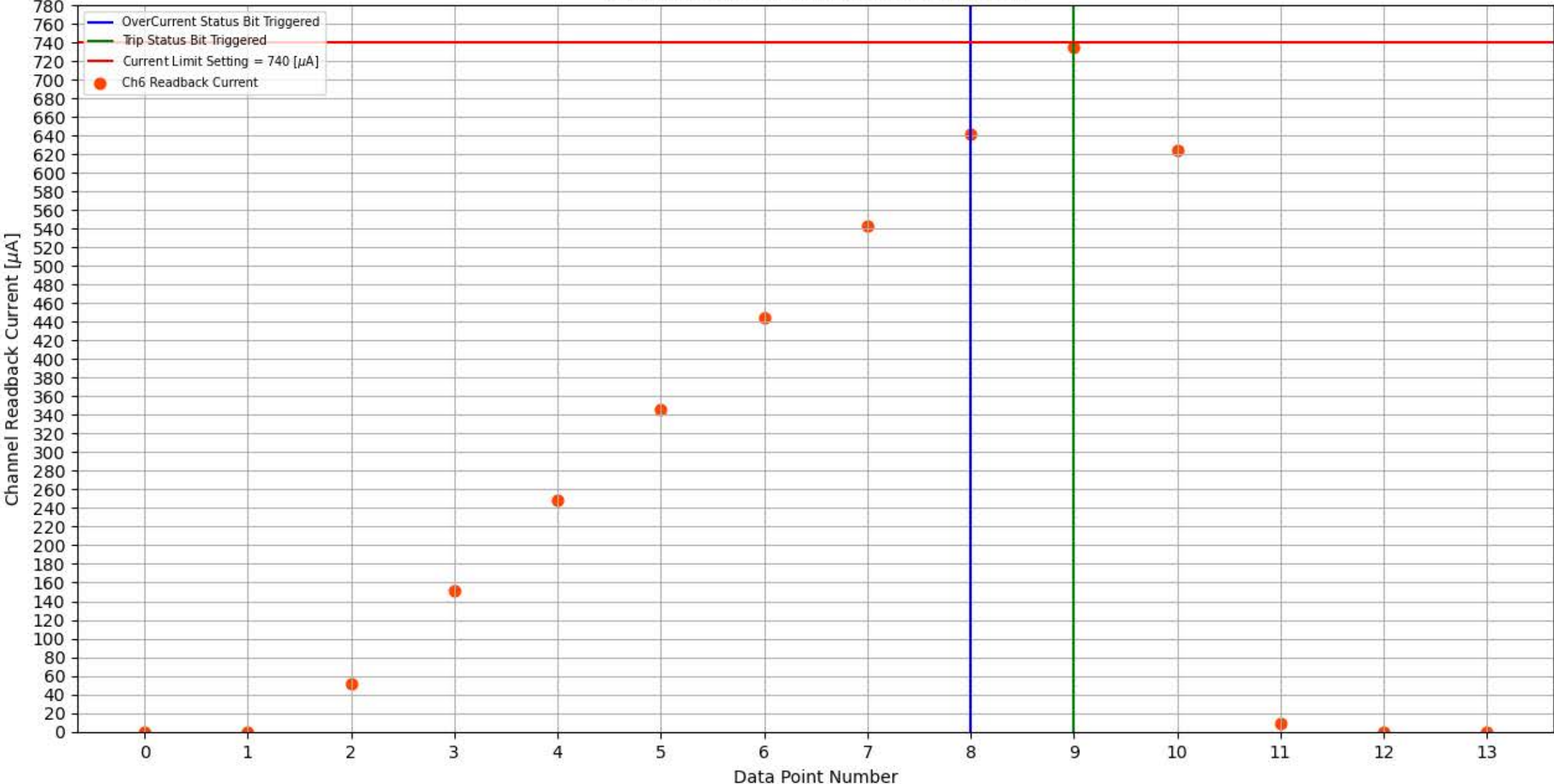
Module 339, Slot 10, Channel 6 Trip Test
