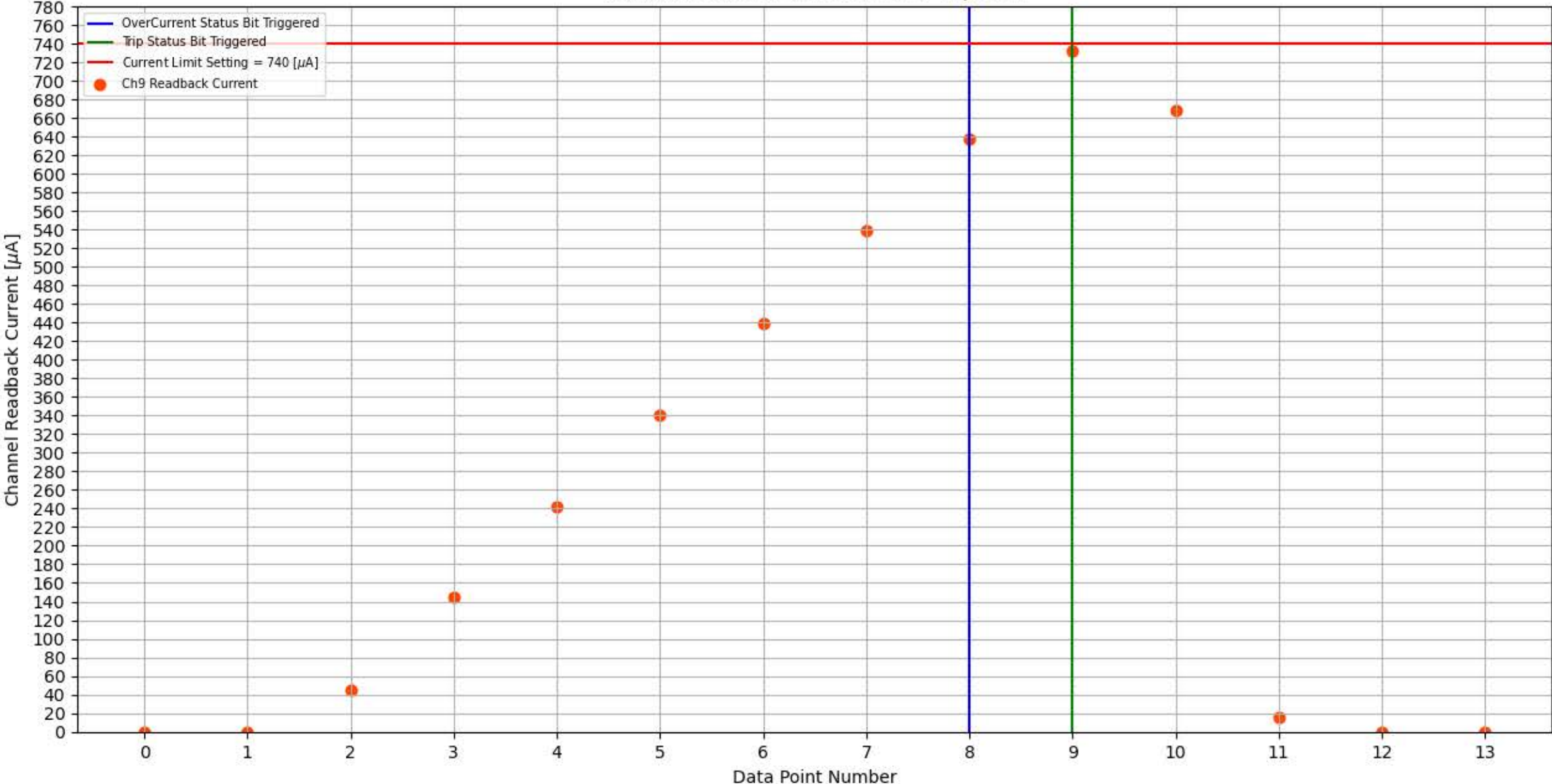
Module 339, Slot 10, Channel 9 Trip Test
