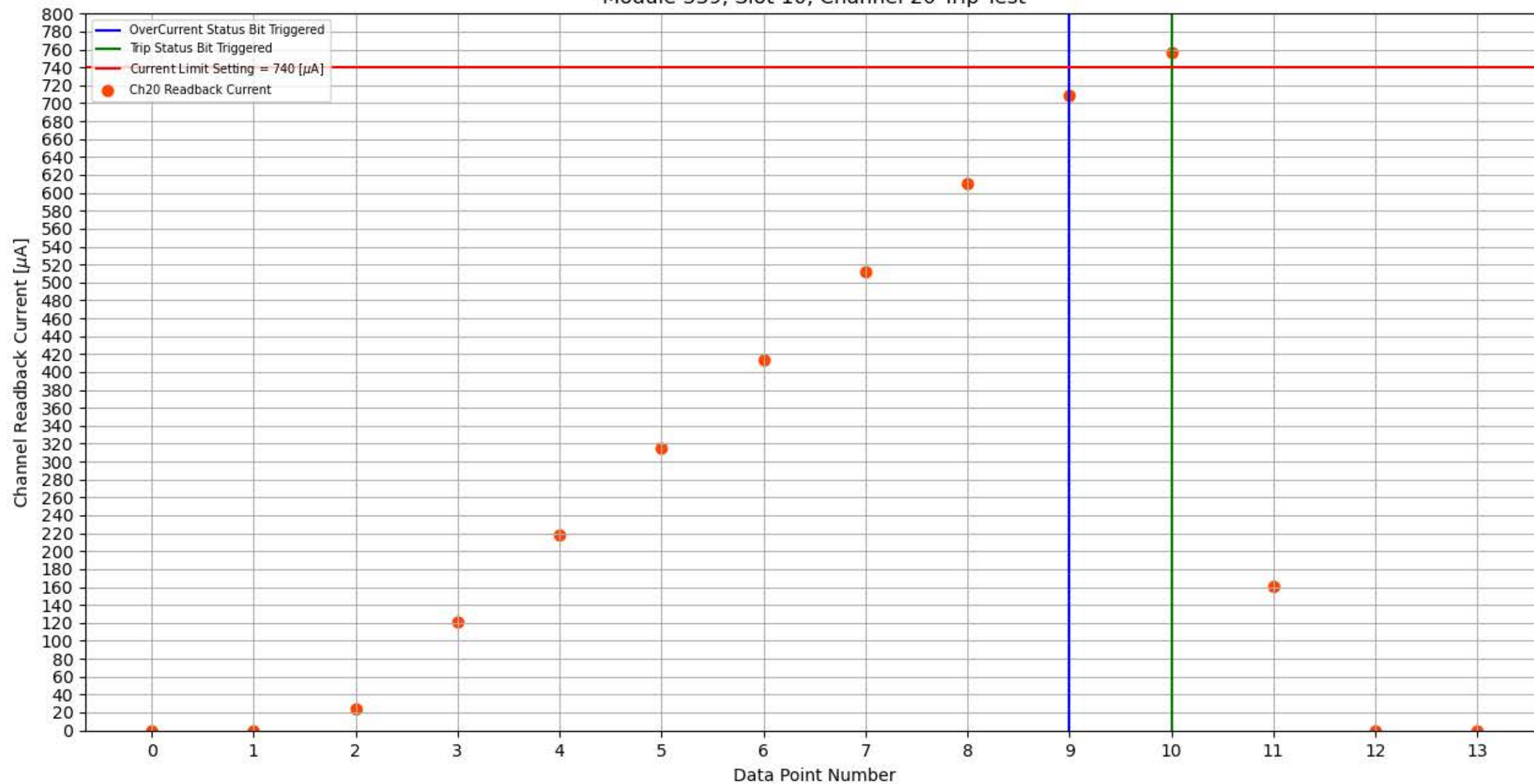
Module 339, Slot 10, Channel 20 Trip Test
