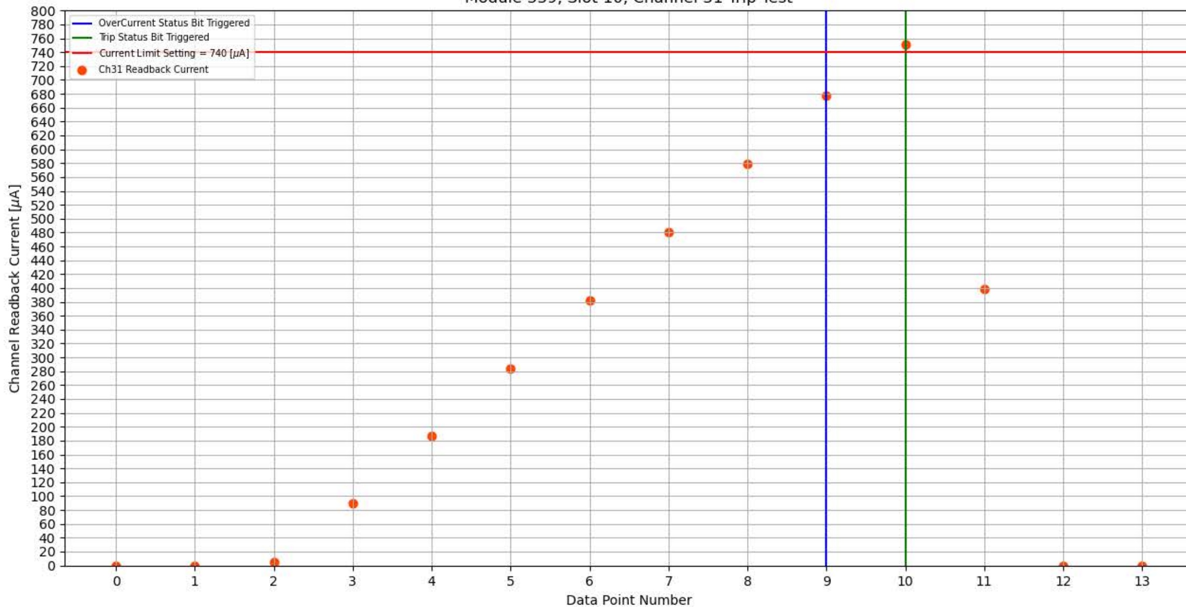
Module 339, Slot 10, Channel 31 Trip Test
