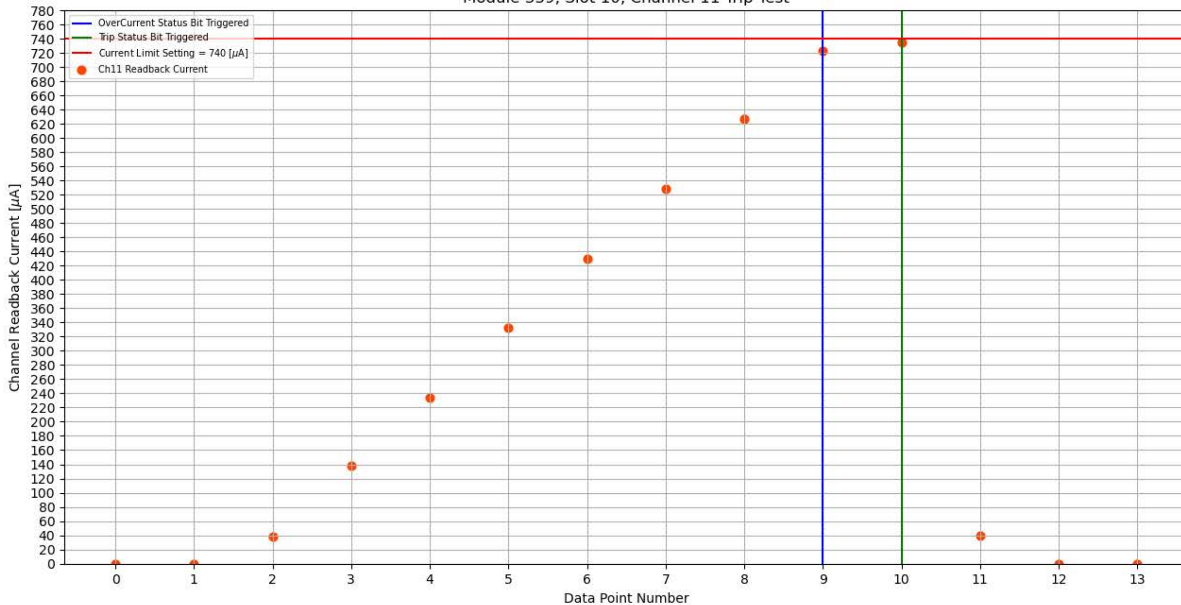
Module 339, Slot 10, Channel 11 Trip Test
