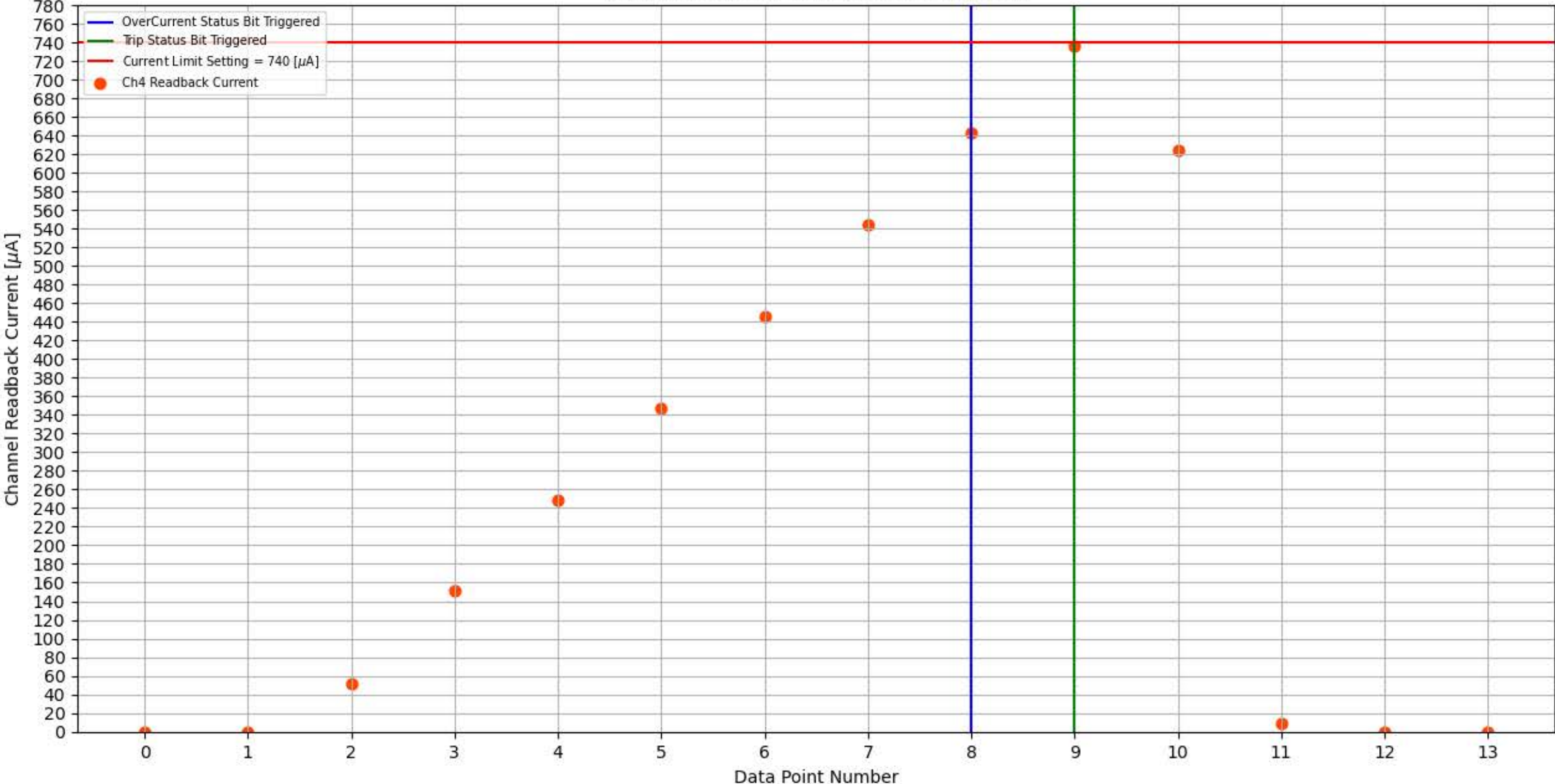
Module 339, Slot 10, Channel 4 Trip Test
