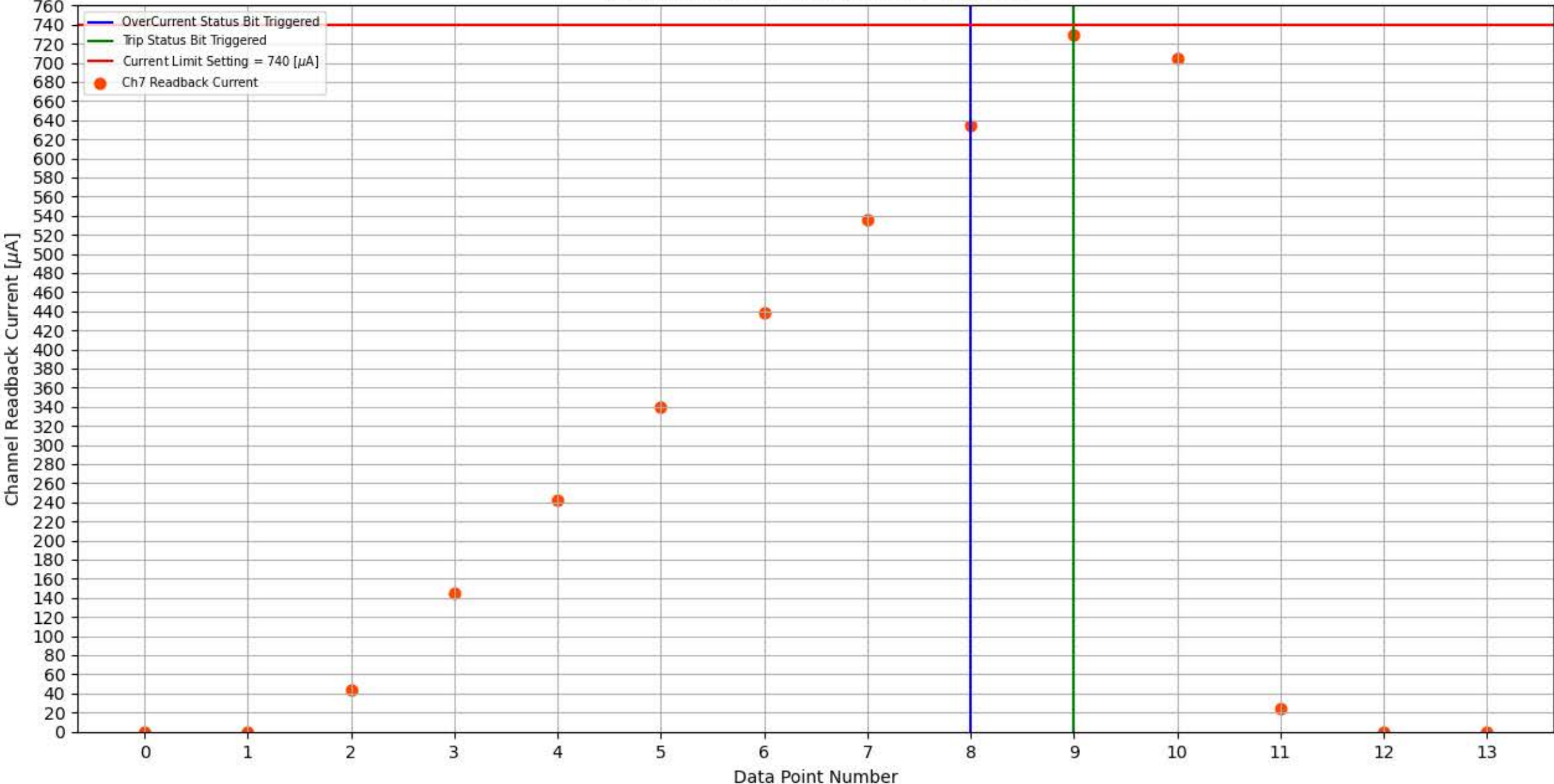
Module 339, Slot 10, Channel 7 Trip Test
