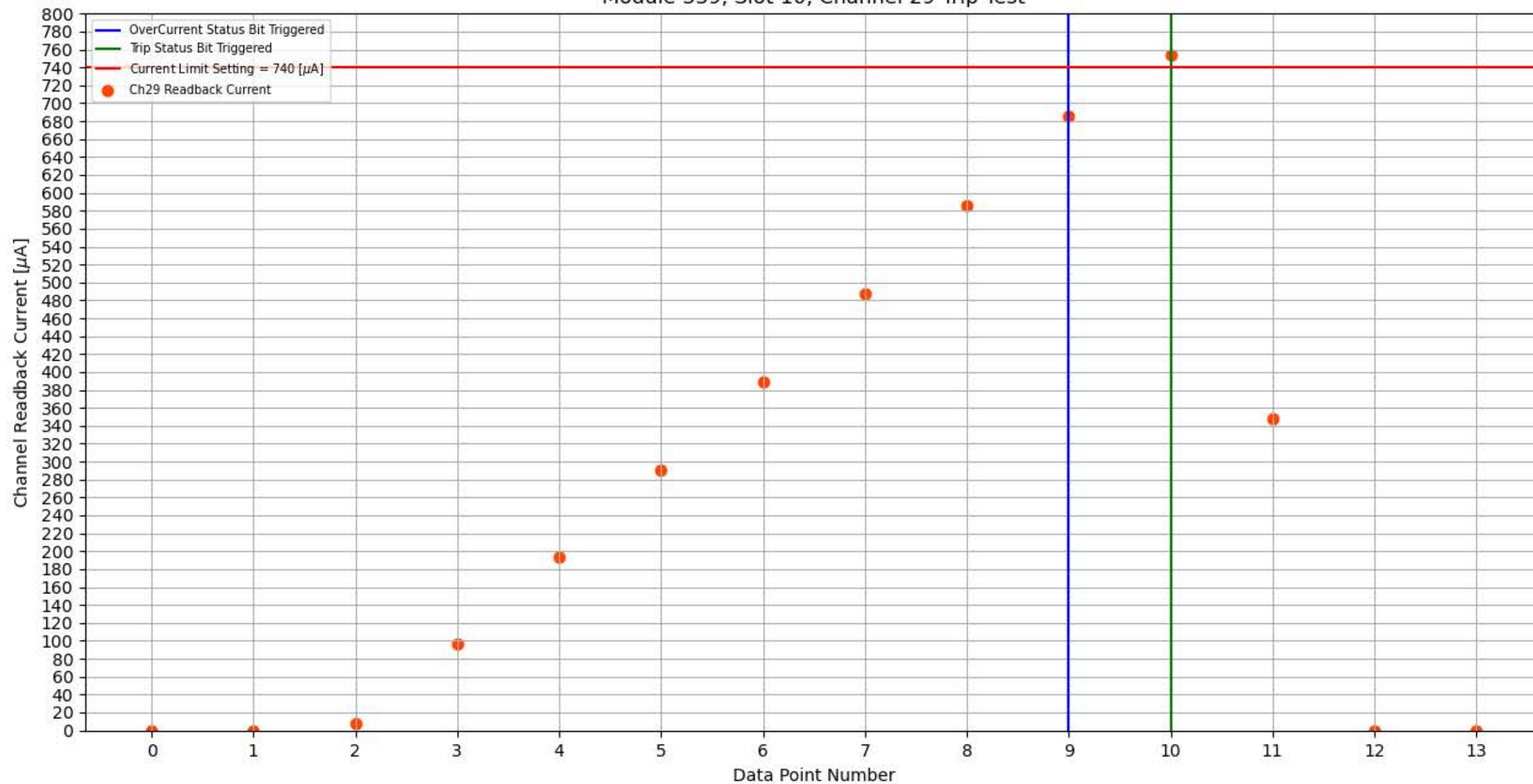
Module 339, Slot 10, Channel 29 Trip Test
