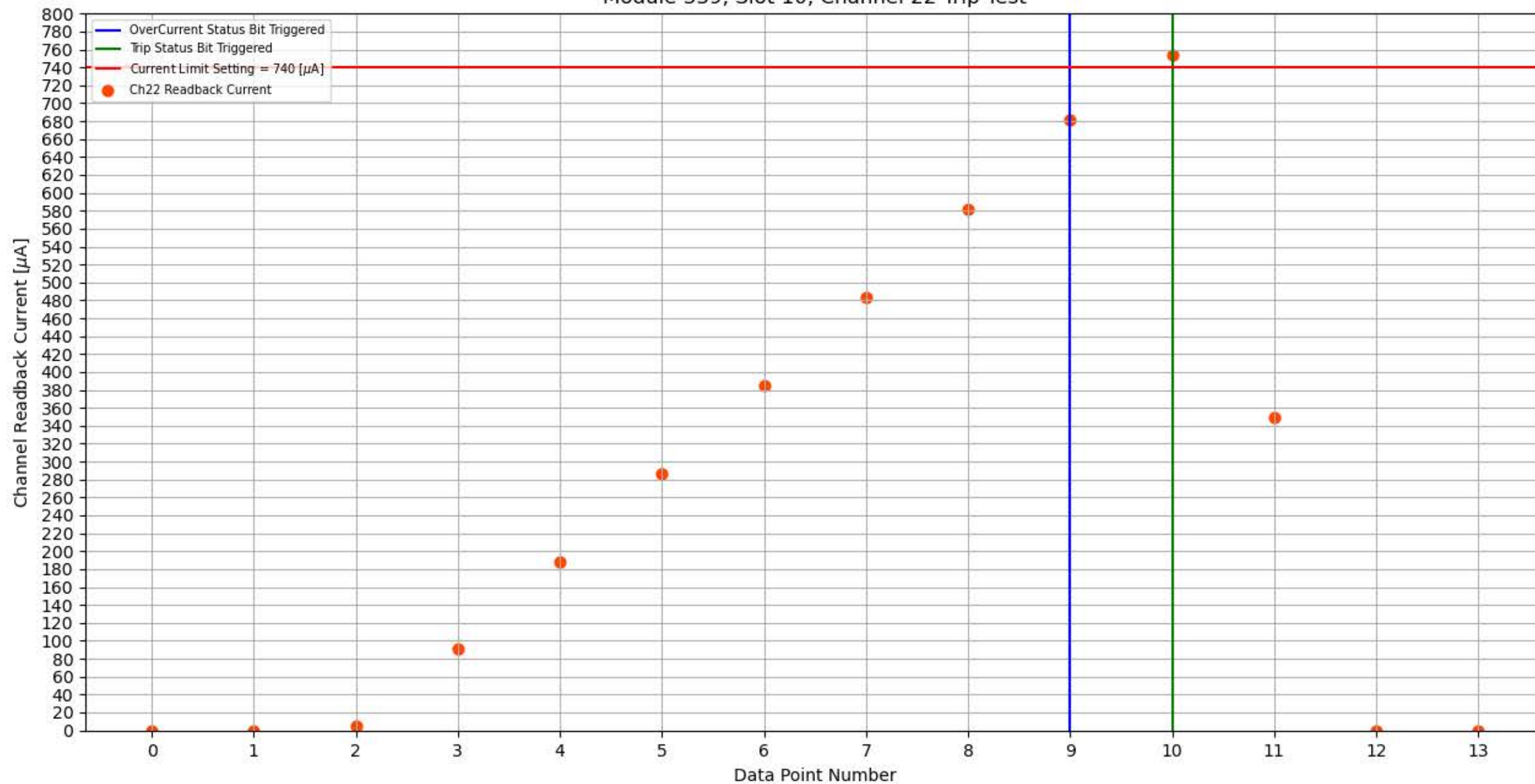
Module 339, Slot 10, Channel 22 Trip Test
