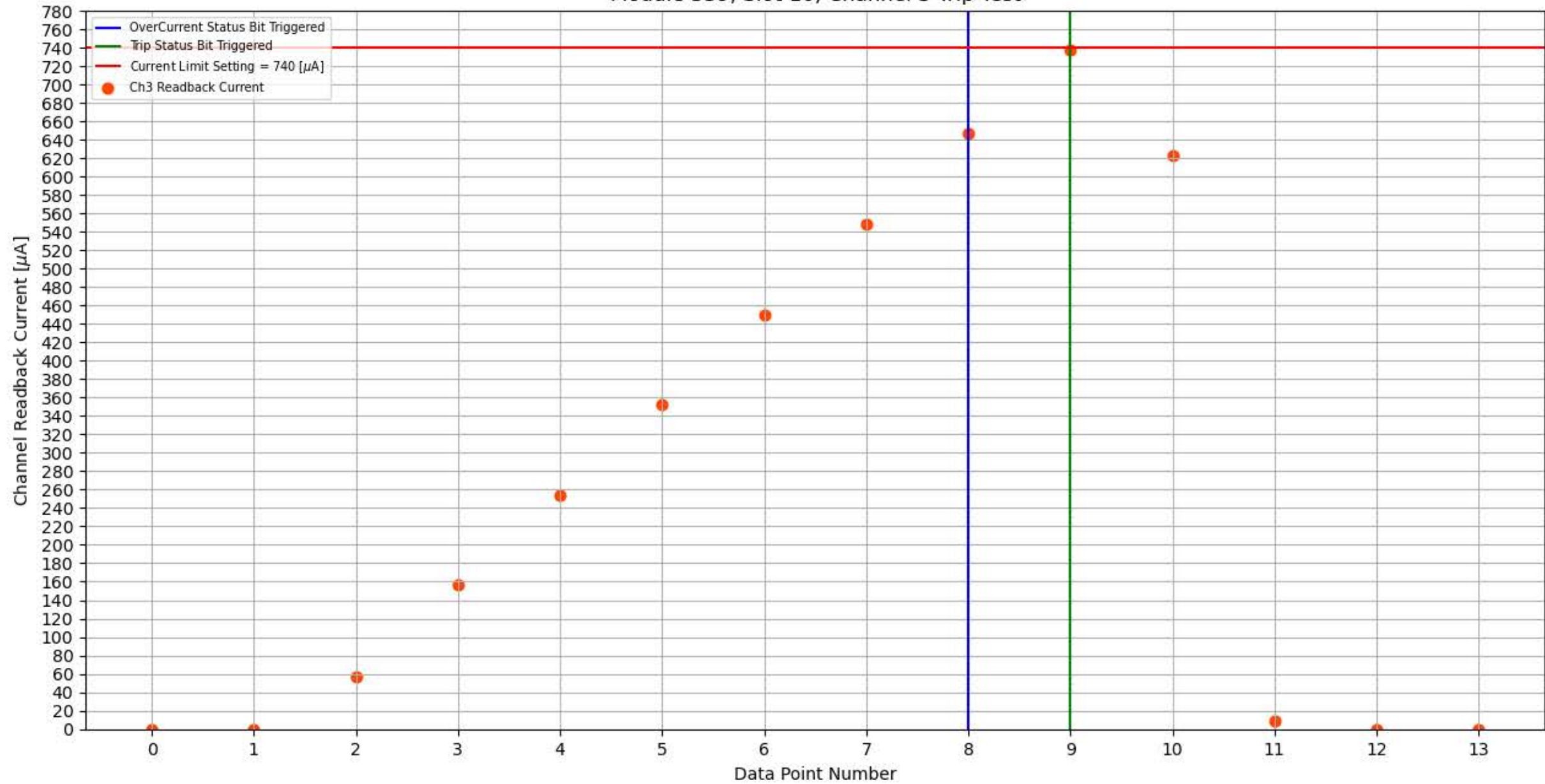
Module 339, Slot 10, Channel 3 Trip Test
