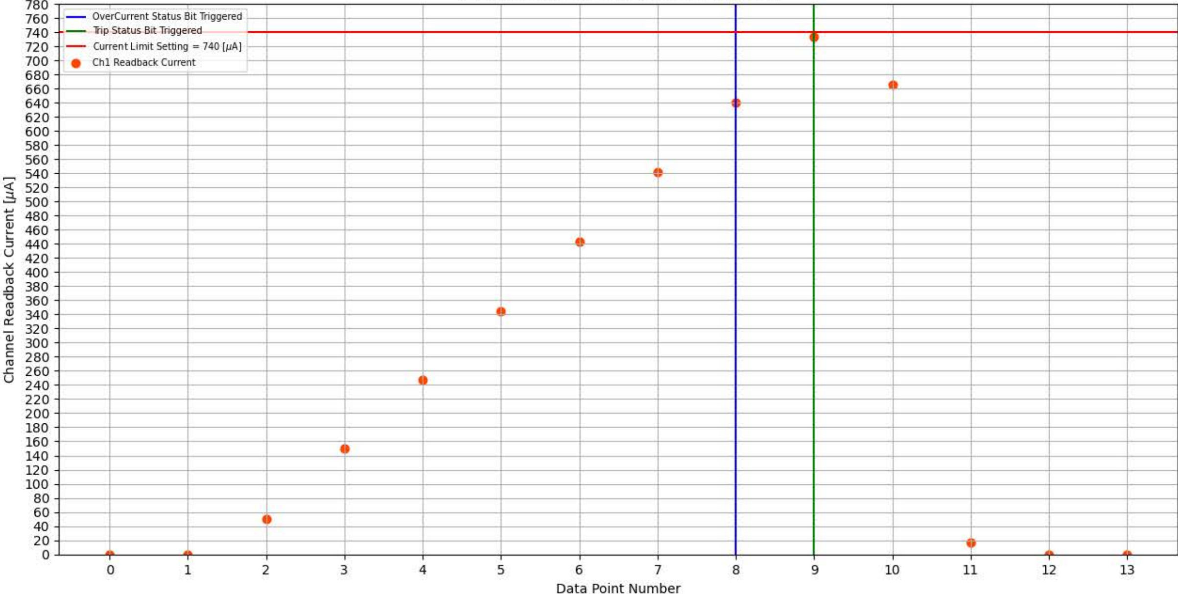
Module 339, Slot 10, Channel 1 Trip Test
