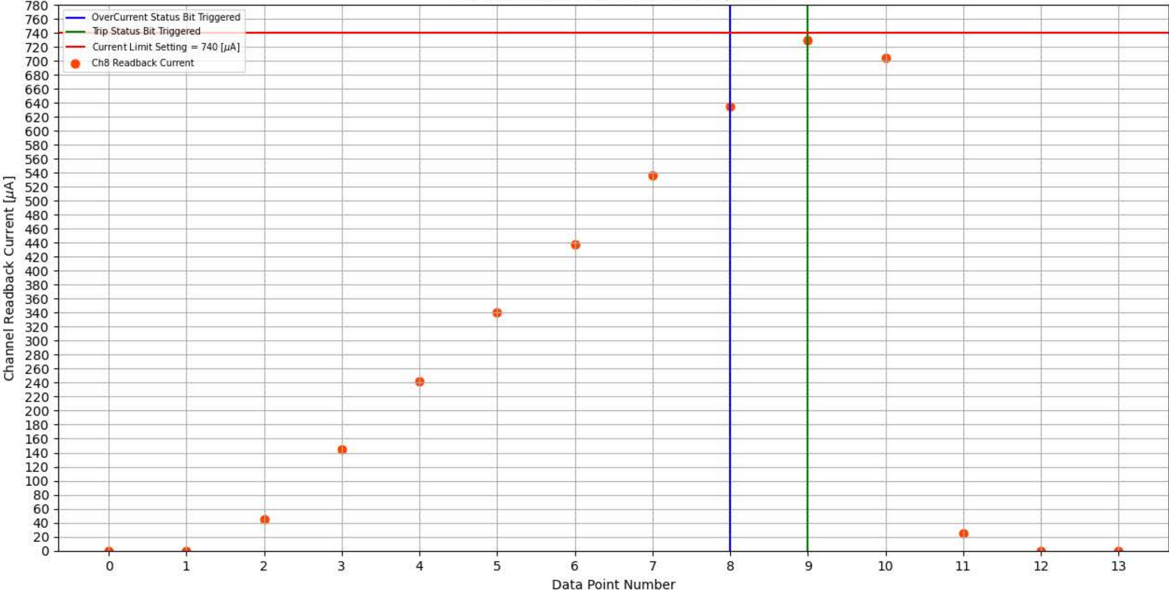
Module 339, Slot 10, Channel 8 Trip Test
