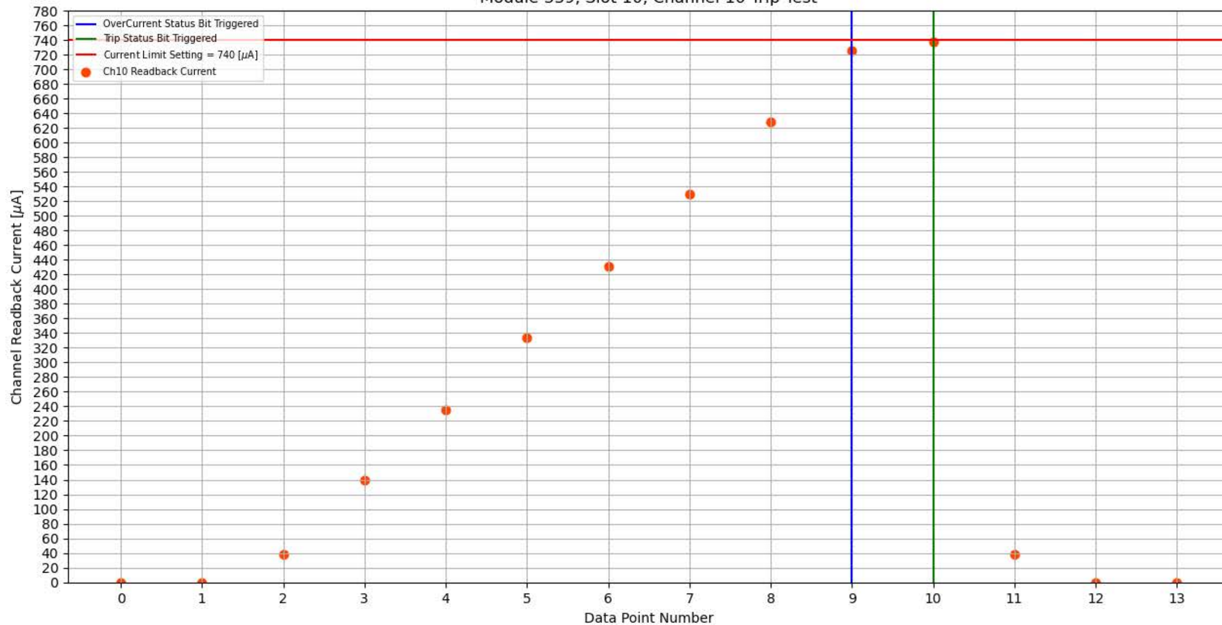
Module 339, Slot 10, Channel 10 Trip Test
