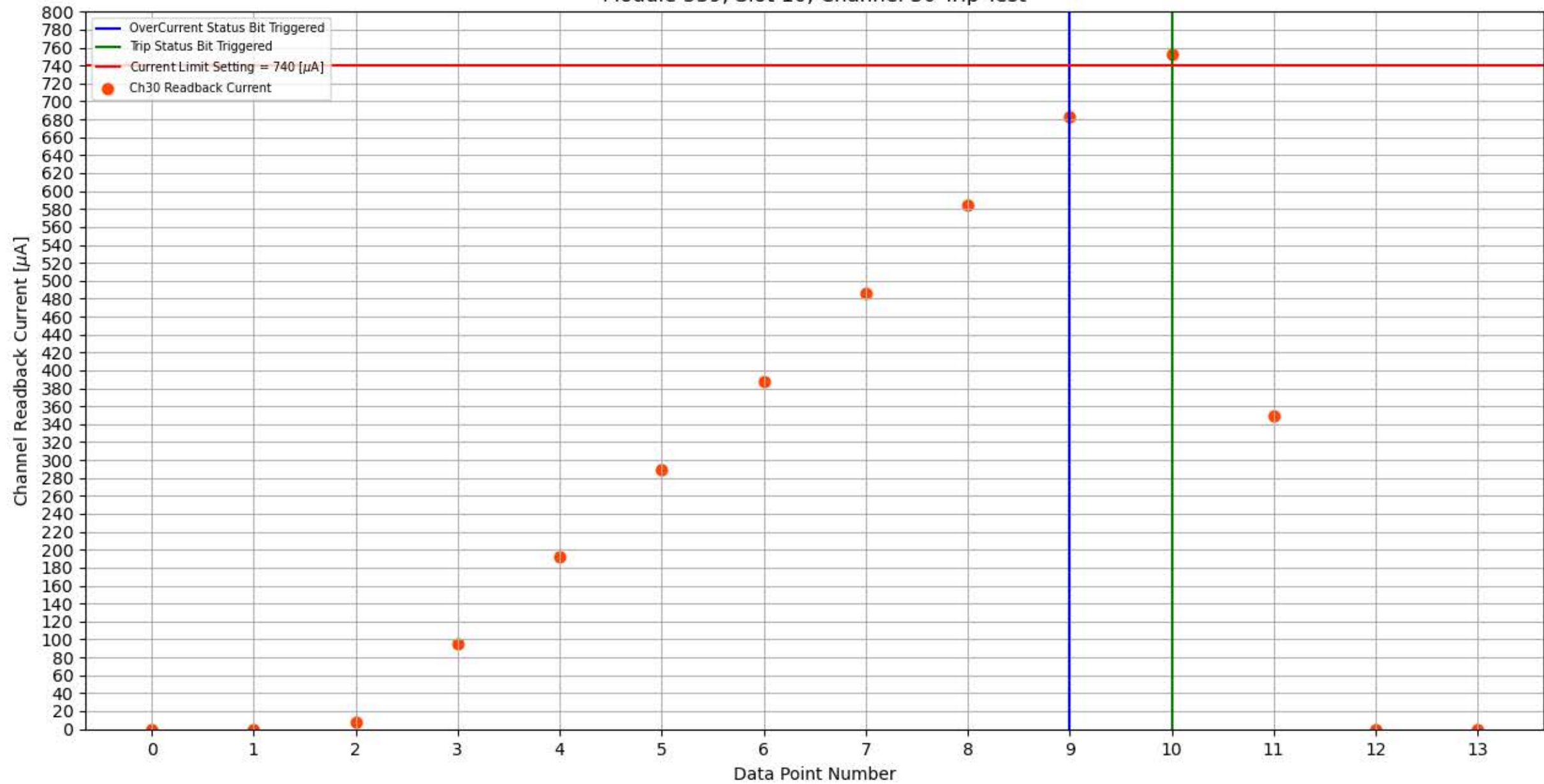
Module 339, Slot 10, Channel 30 Trip Test
