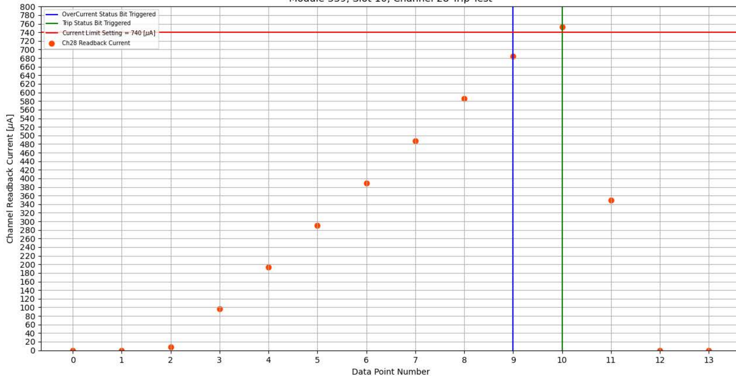
Module 339, Slot 10, Channel 28 Trip Test
