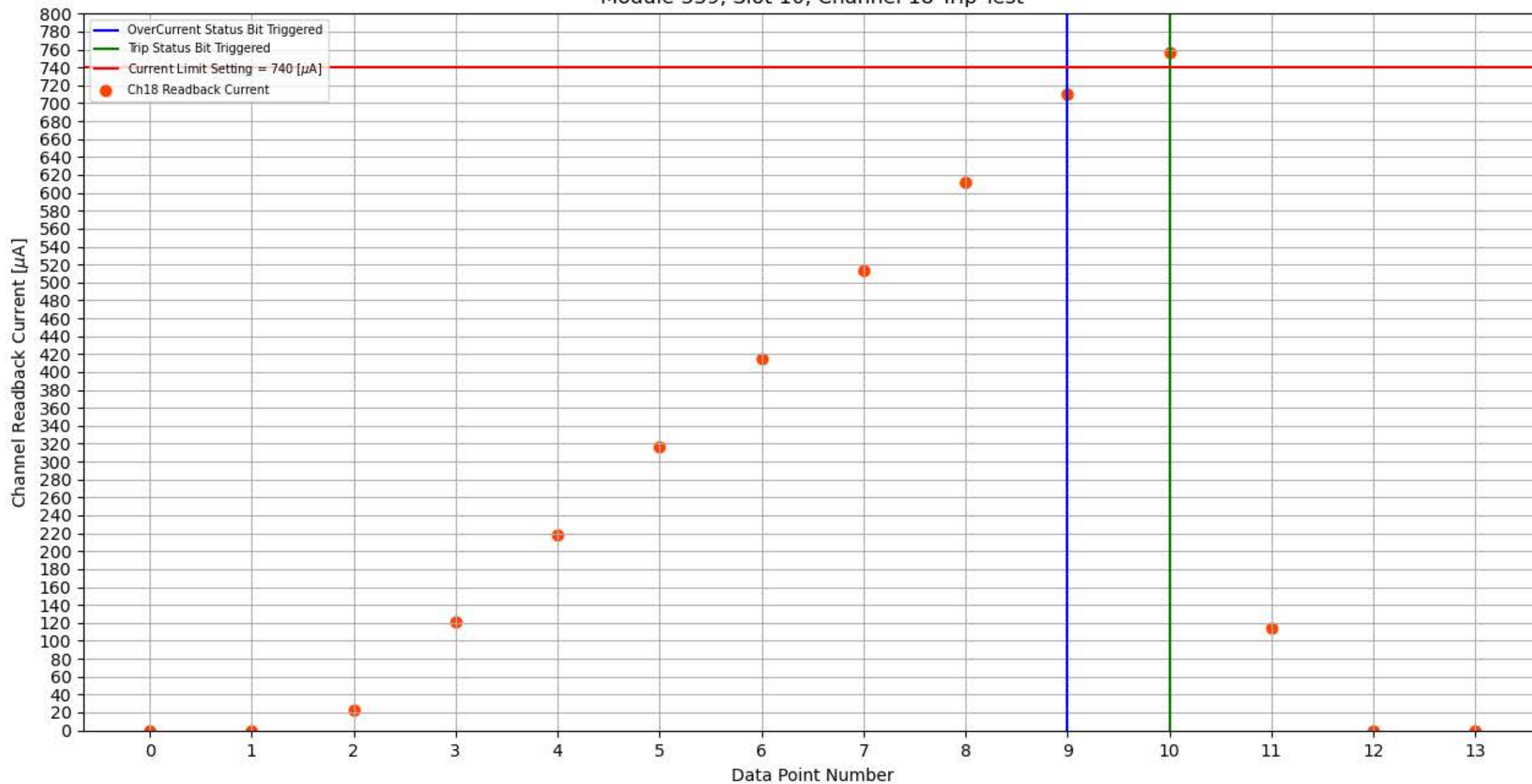
Module 339, Slot 10, Channel 18 Trip Test
