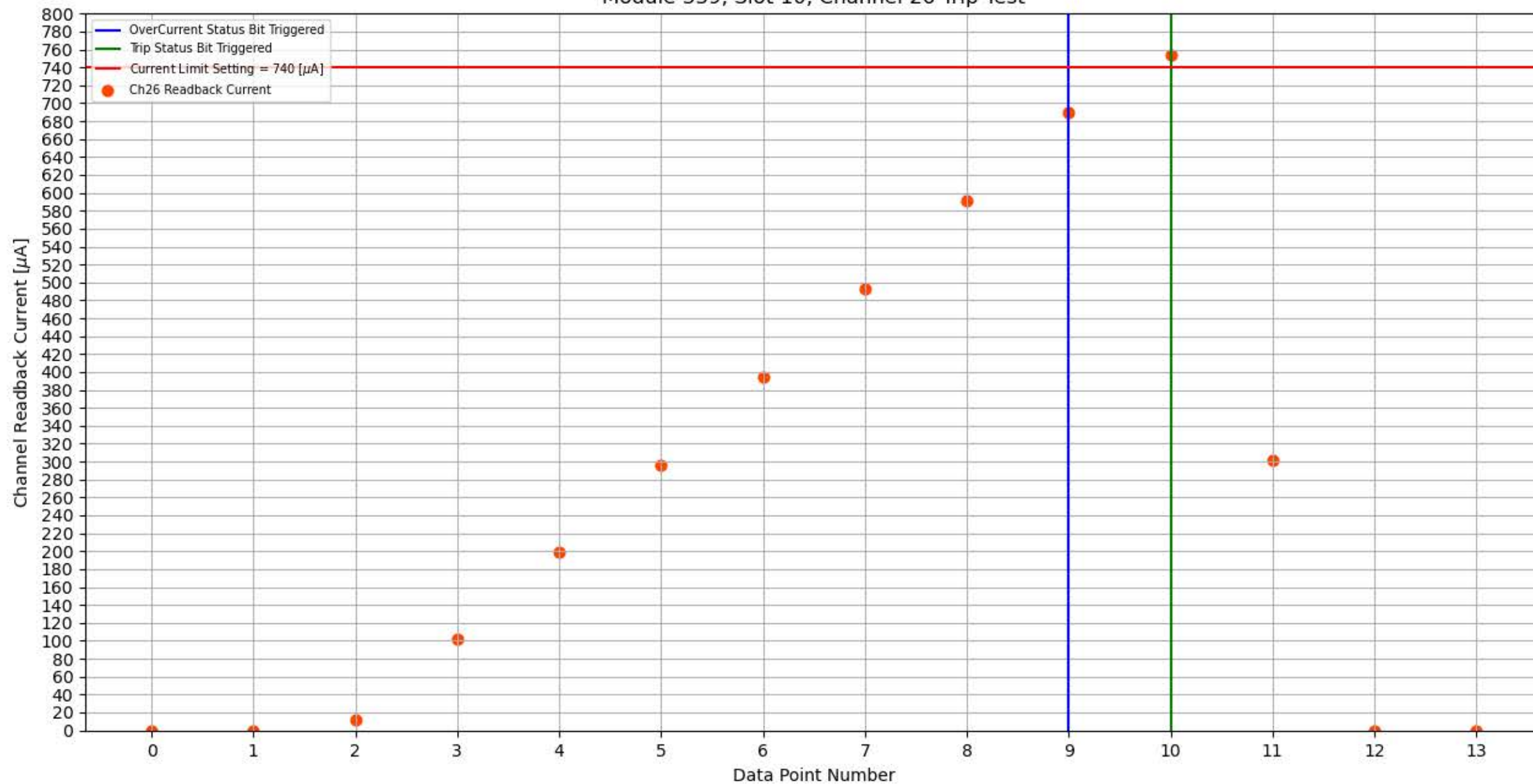
Module 339, Slot 10, Channel 26 Trip Test
