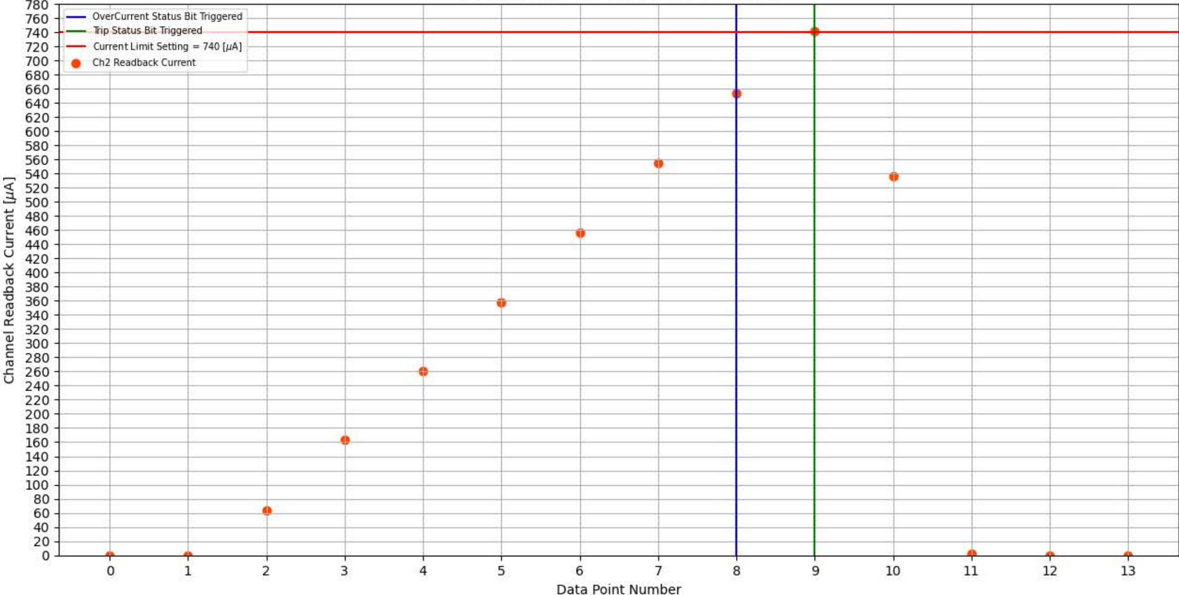
Module 339, Slot 10, Channel 2 Trip Test
