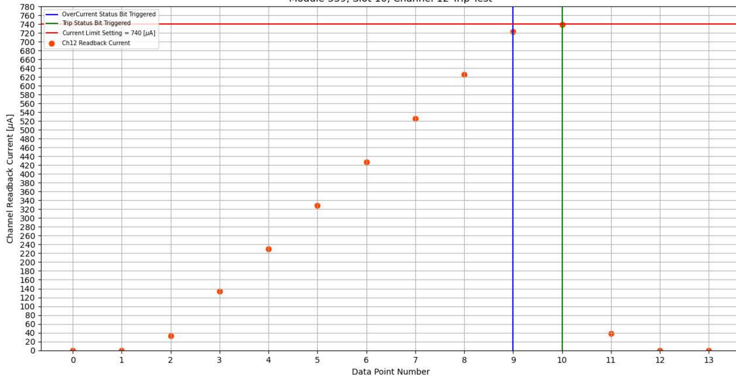
Module 339, Slot 10, Channel 12 Trip Test
